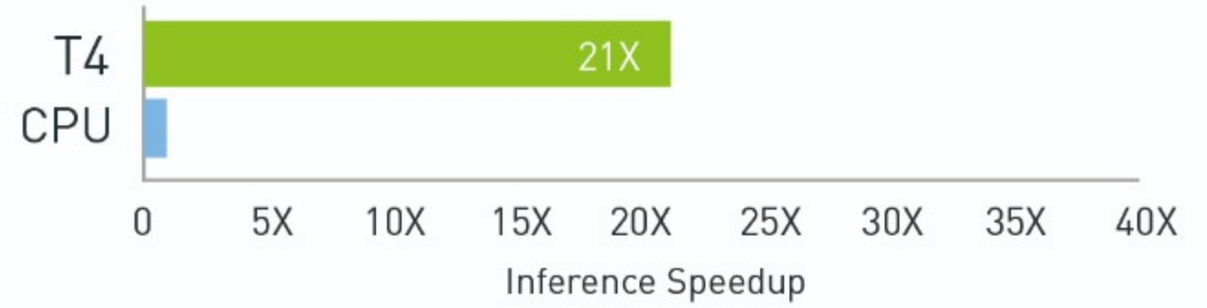
DeepSpeech2
